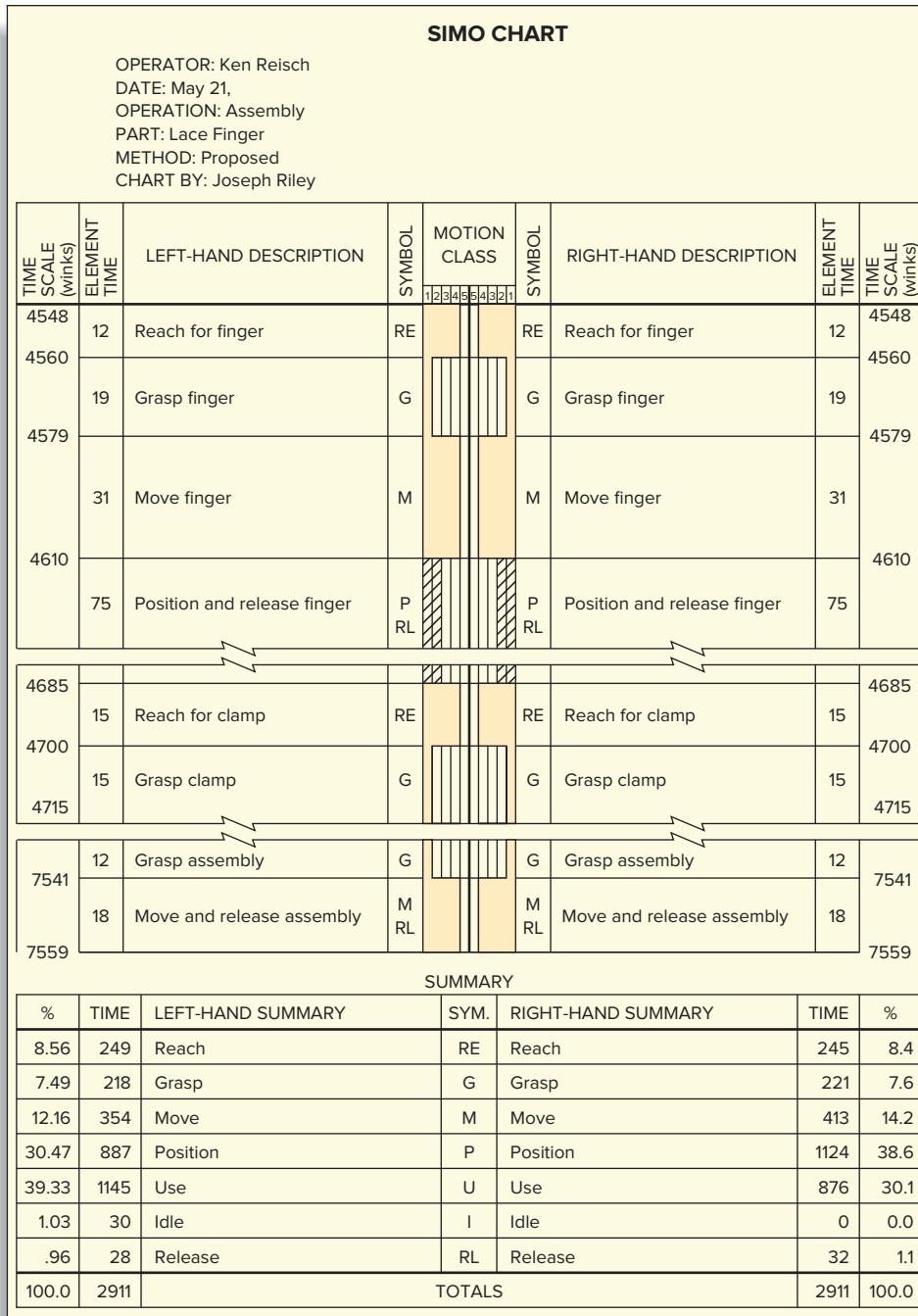
FIGURE 7.6 A simultaneous motion chart
