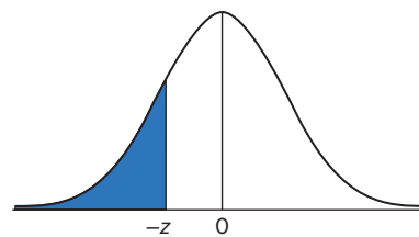
FIGURE C.2 The standard normal distribution with selected values of z
