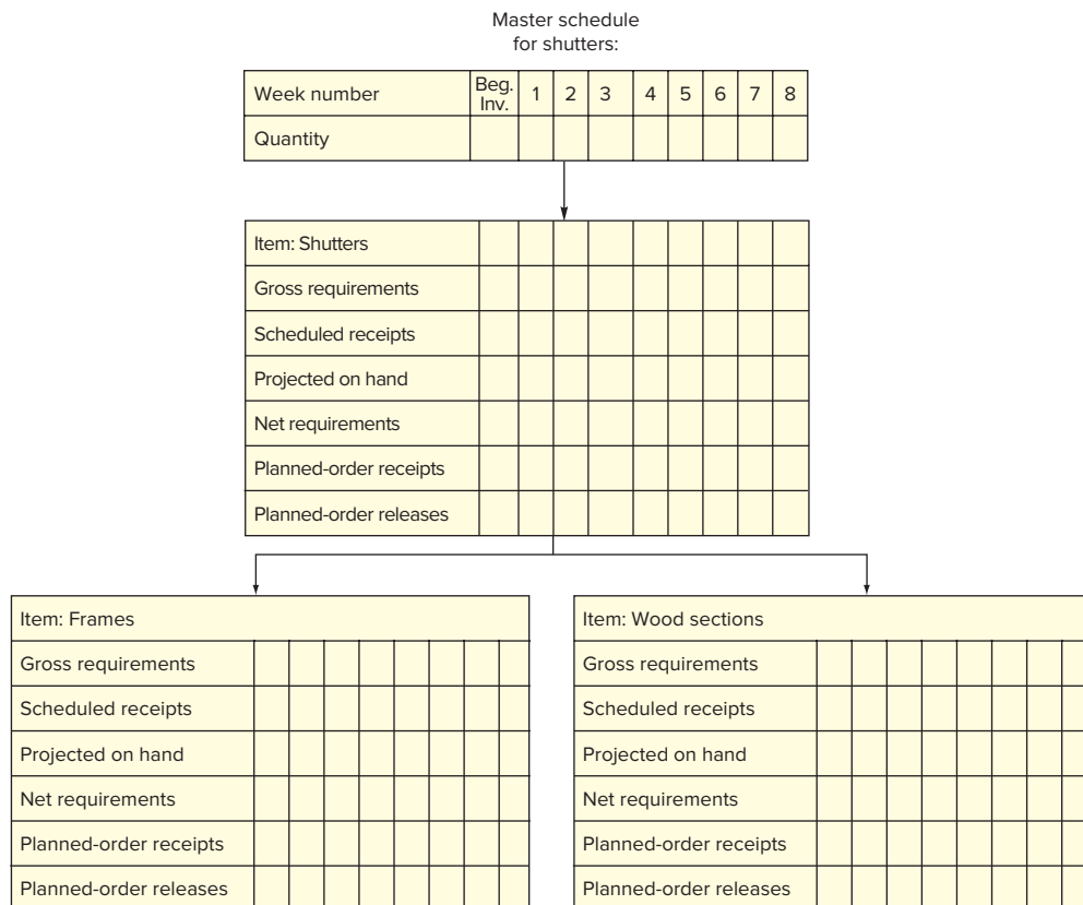
FIGURE 13.10 Net requirements at each level determine gross requirements at the next.
