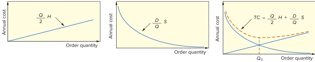
FIGURE 12.4 Carrying cost, ordering cost, and total cost curve
