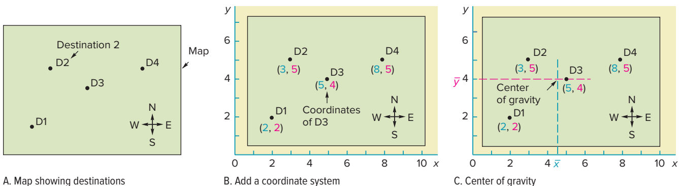
FIGURE 8.1 Center-of-gravity method
