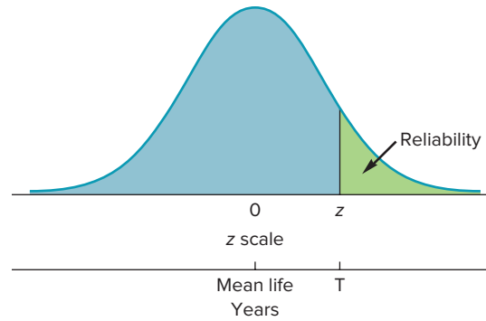
FIGURE 4S.3 A normal curve
