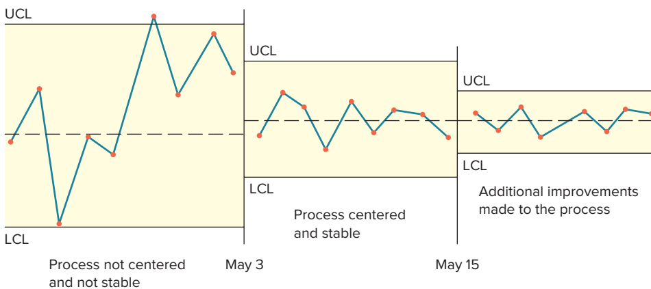
FIGURE 9.14 Using a control chart to track improvements
