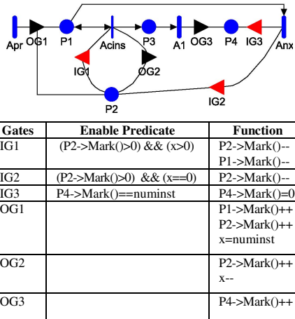
Fig. 7. SAN submodel for multiple instance with a prior, design time knowledge
