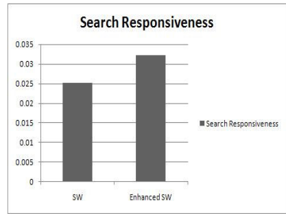
Fig. 4. Search Responsiveness
