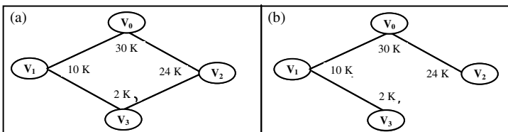
Fig. 1. Complete Lattice and Reduced Lattice
