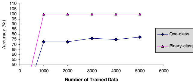
Fig. 6. One-class and Binary classification comparison
