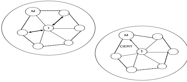
Fig. 3. (a) Trust Information Collection (b) Trust Certificate Generation
