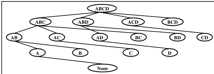
Fig. 4. Reduced Lattice
