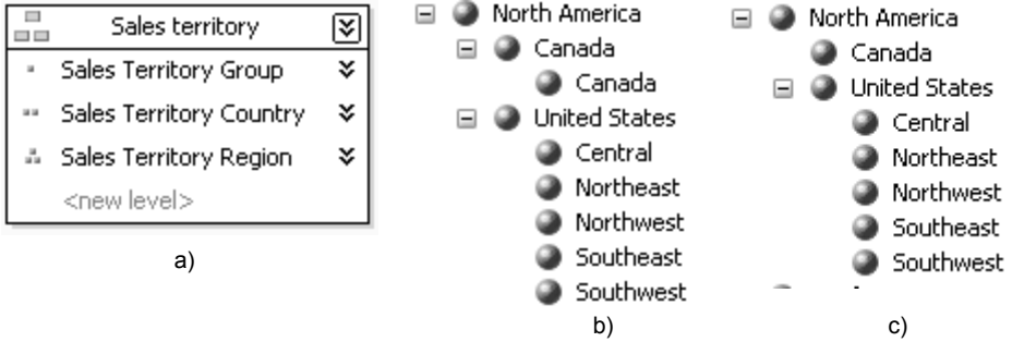
Fig. 4. Unbalanced hierarchy in SSAS: a) schema and b), c) instances
