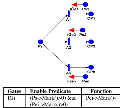
Fig. 5. SAN submodel for deferred choice
